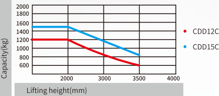
CAPACITY CHART
